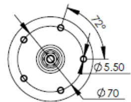
Relevant mounting dimensions on part
